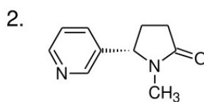
(-)-Cotinine
